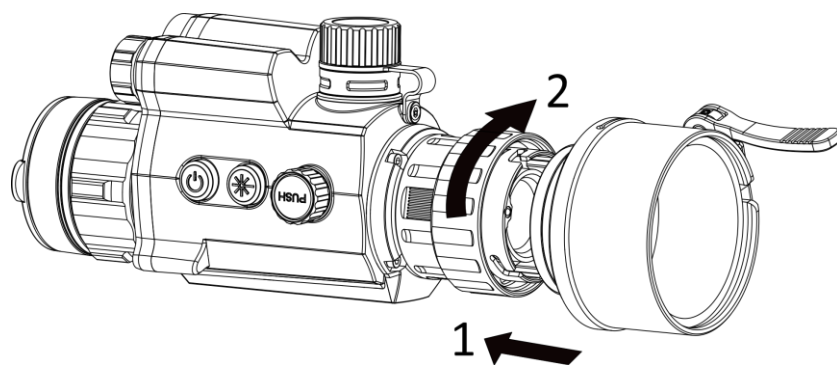
Figure 2-2 Install Adapter
