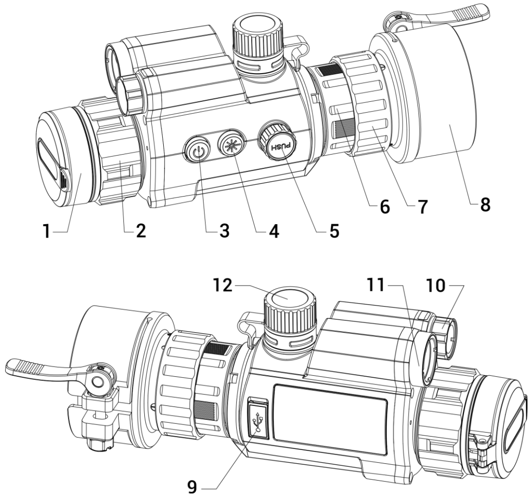
Figure 1-1 Device Appearance
