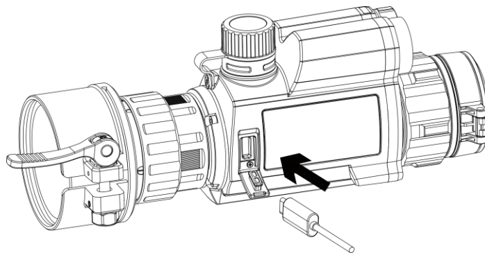
Figure 2-1 Cable Connection
